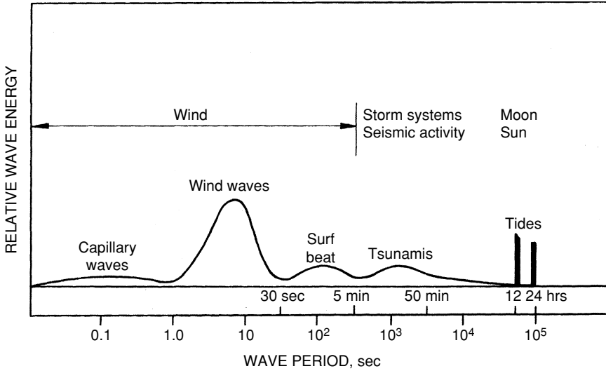
Figure 5.2. Typical ocean wave energy spectrum.
