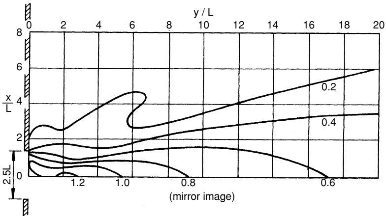
Figure 4.11. K_d values for the lee of a barrier gap 2.5 wave lengths wide, with normally incident waves. (Johnson, 1952.)
